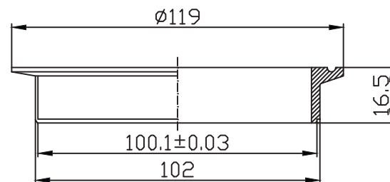
4" weld ferrule
